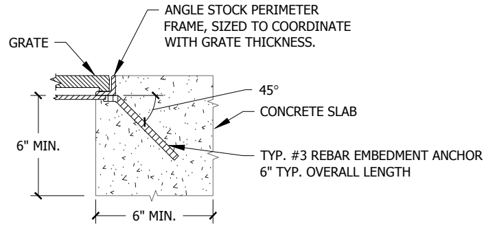
Detail Elevation A-A
