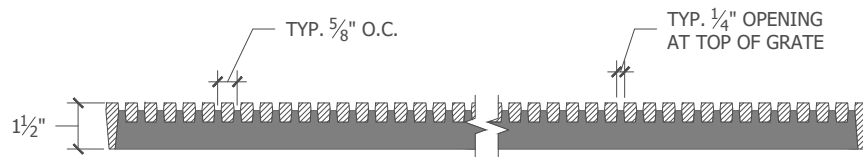
Section B-B'
