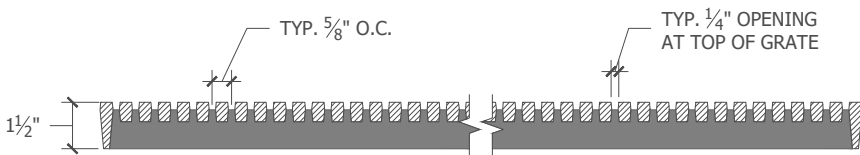
Section B-B'
