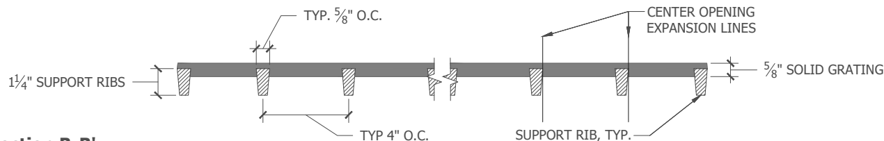
Section B-B'
