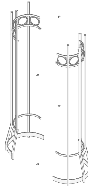
Exploded Isometric
