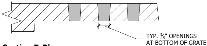
Section B-B'
