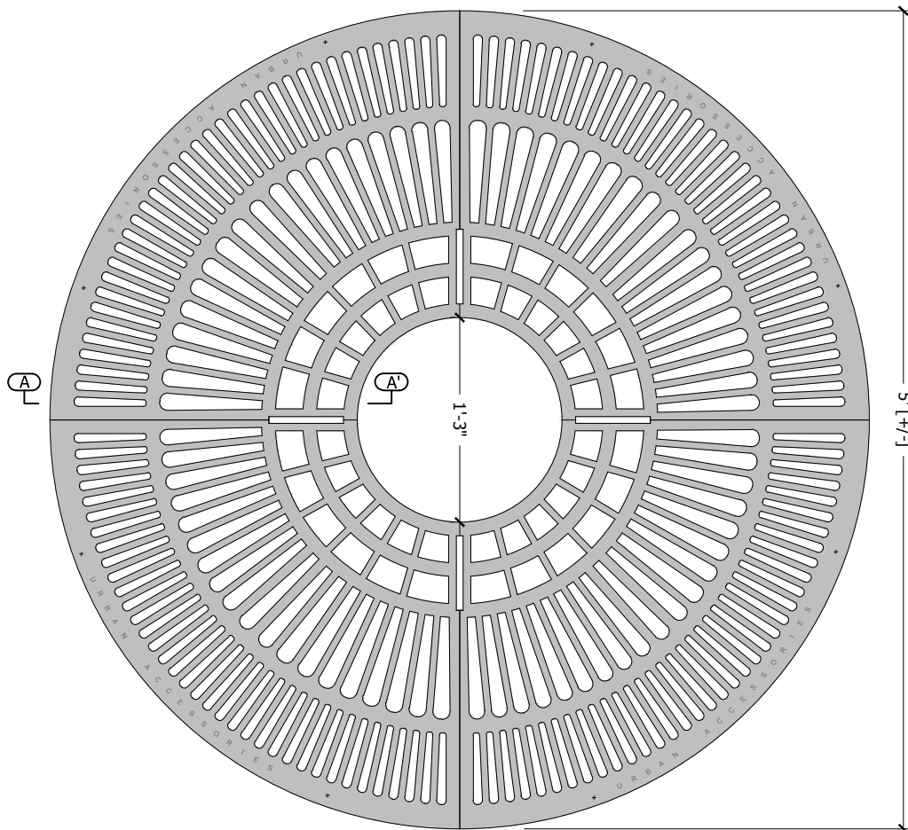
Plan
