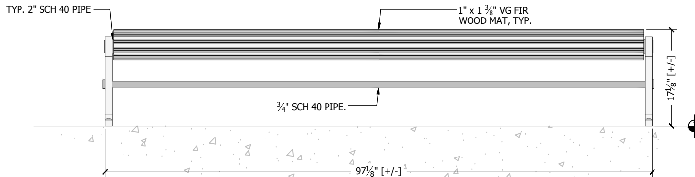
Front View
