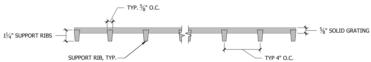
Section B-B'
