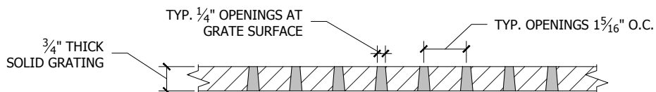
Section B-B'
