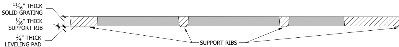
Section C-C'
