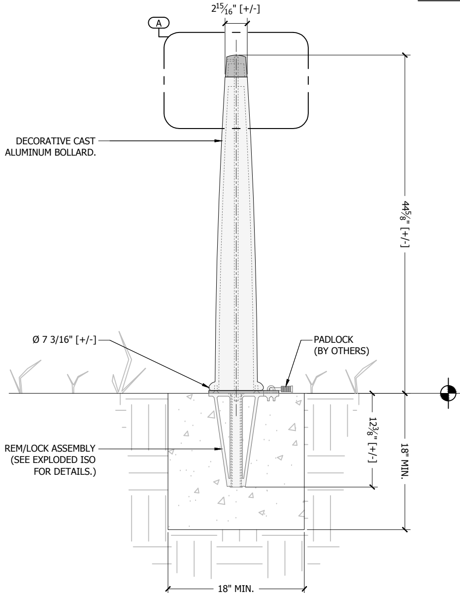
Detail A
