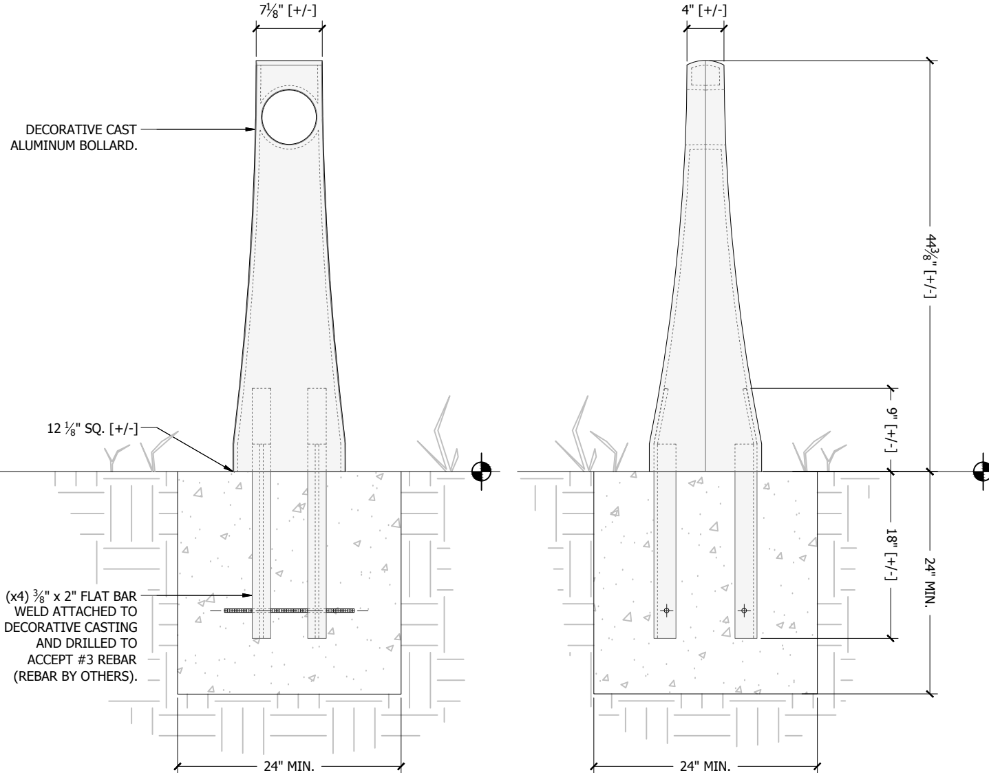
Front View
