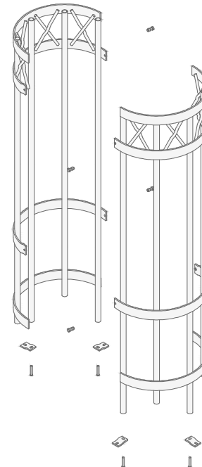
Exploded Isometric
