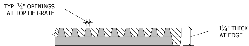
Section B-B'
