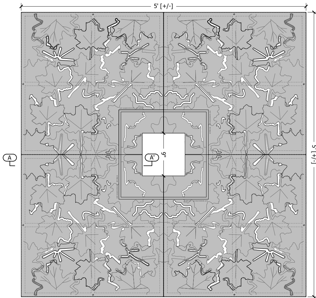
Plan
