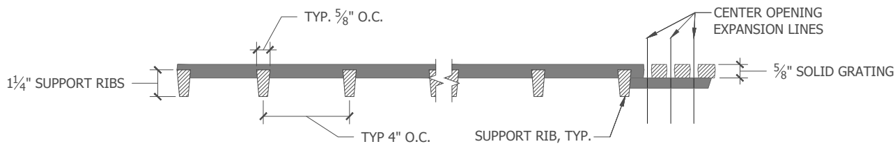
Section B-B'
